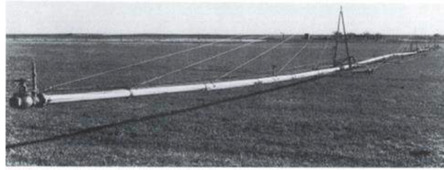
ORIGINAL CENTER-PIVOT MACHINE, invented by Frank Zybach some 25 years ago, introduced two key innovations that led to the successful development of a completely automatic irrigation system. In Zybach's scheme the pipe supplying water to conventional sprinkler nozzles is supported by a series of Adams towers. The system is propelled by means of water hauled from the supply line (see illustration below).
