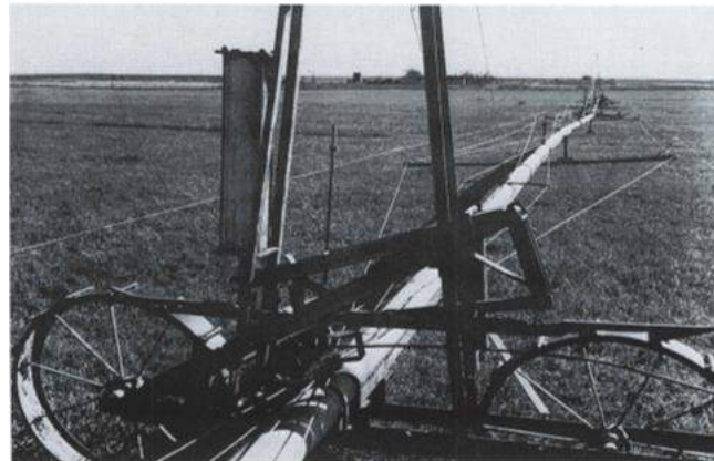
CLOSE-UP of one of the mobile towers of the original center-pivot machine shows the parts of the system with greater clarity. Water taken under pressure from the supply line powers a piston, which
